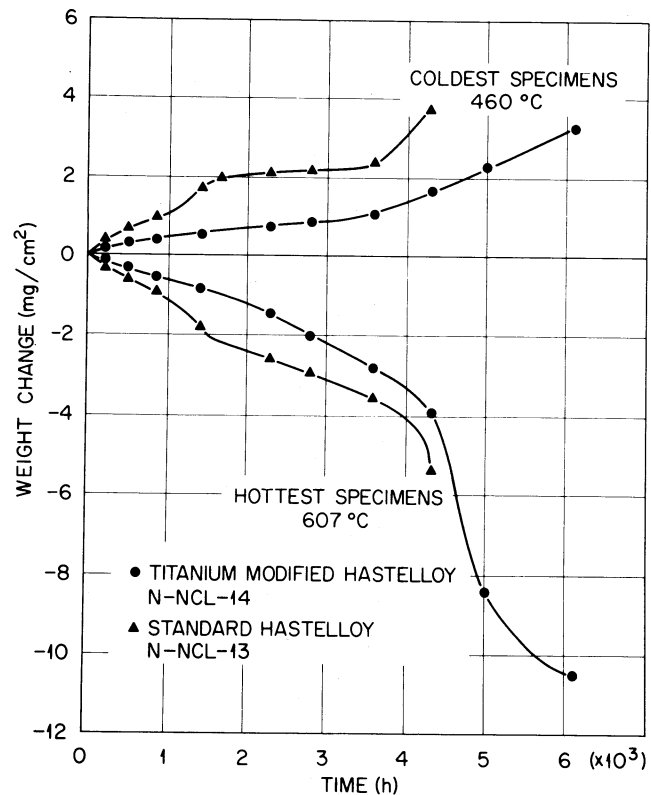
Fig. 12. Comparison of the weight changes of Hastelloy-N specimens inserted in \text{NaBF}_4 - \text{NaF} (92-8 mole%) thermal convection loops. (Assuming uniform corrosion, a weight change of 20 mg/cm 2 in 8750 h is equivalent to a corrosion rate of ~1 mil/year.)
