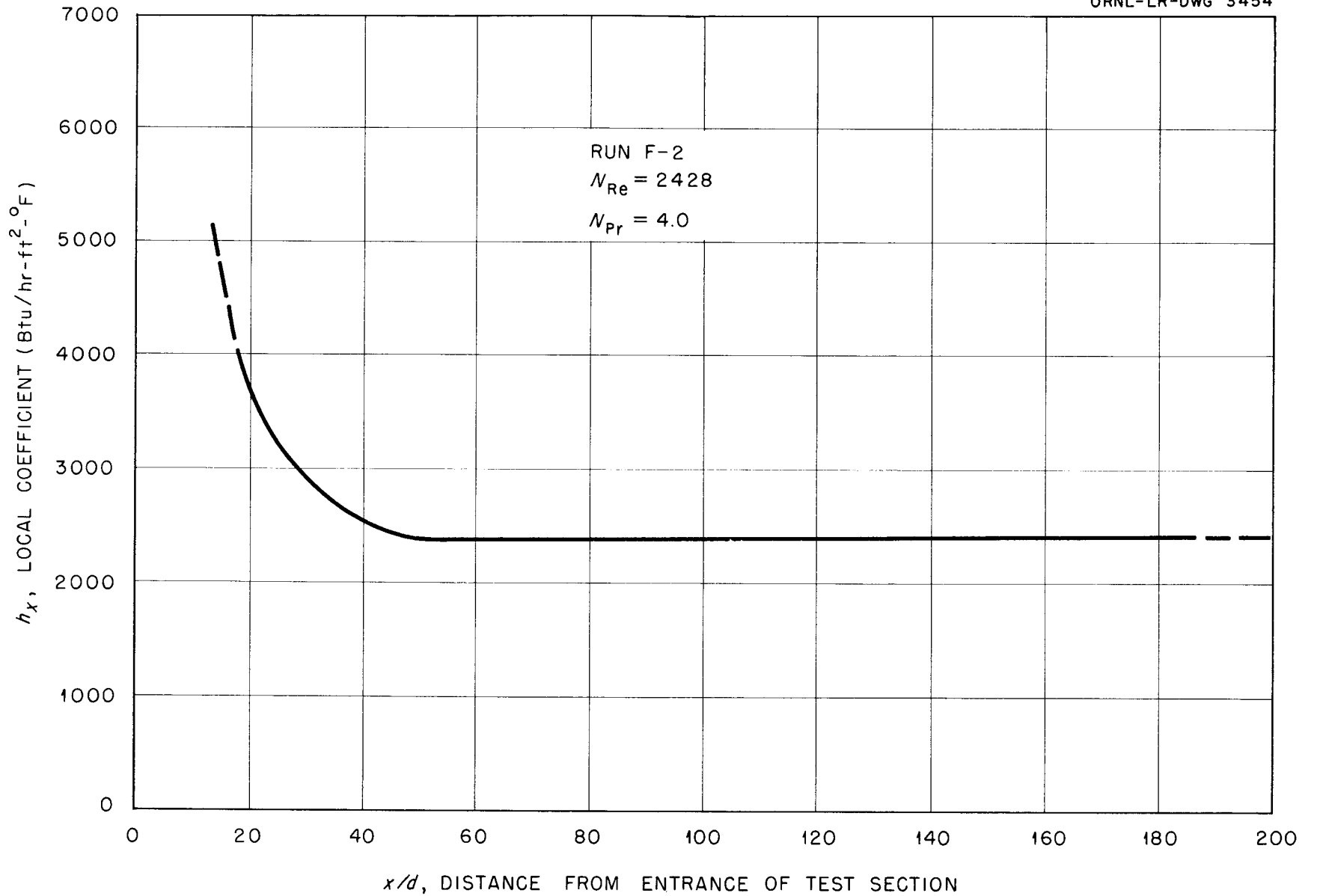
Fig. 10. Local Heat Transfer Coefficients for FLINAK Flowing in a Pipe under Uniform Flux Conditions.
