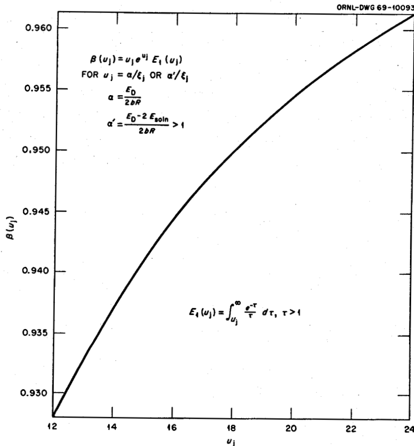
Fig. 7. Plot of \beta(u_j) for Large Values of u_j . The function \beta(u_j) carries contributions of E_1(u_j) ; the interval of u_j is dictated by values of parameters peculiar to the sodium-Inconel 600 system.
