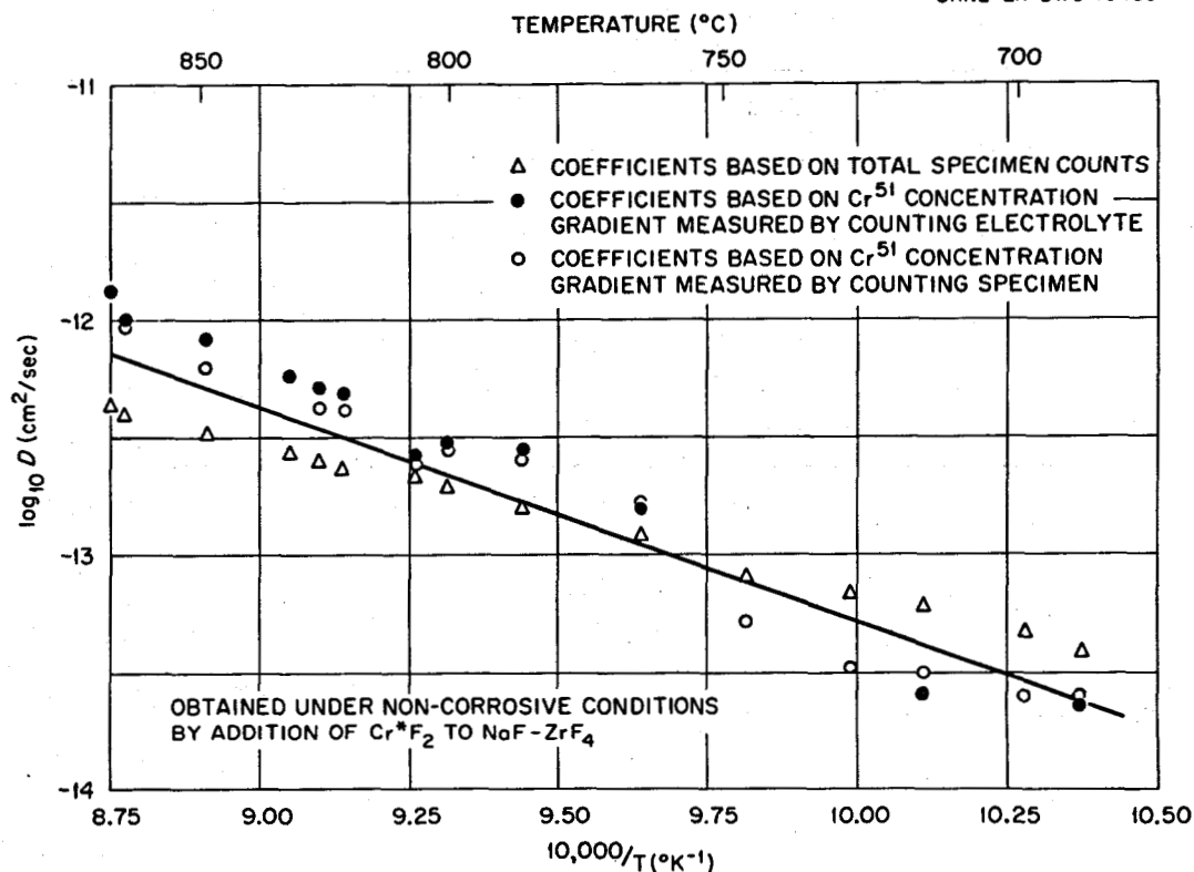
Fig. 12. Diffusion Coefficients of ^{51}\text{Cr} Obtained from a Tracer Loop Experiment (1248 on Fig. 11). The average curve was the basis for D_0 and E_D used in all computations relative to molten-salt examples.
