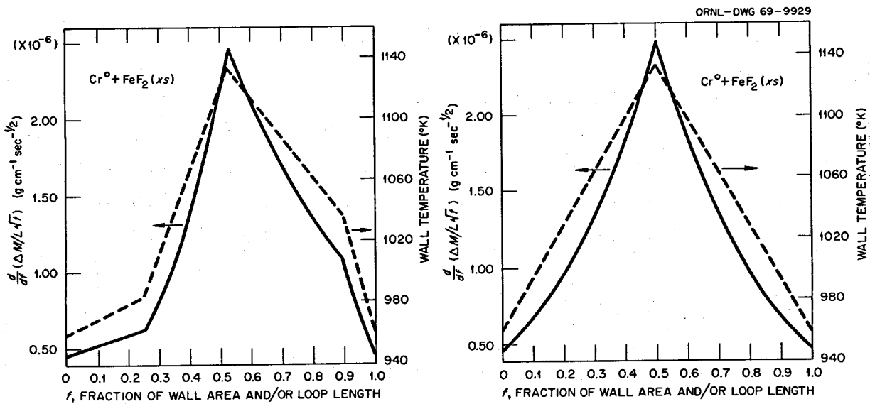
Fig. 13. Profiles for Computed Chromium Corrosion of Hastelloy N when High \text{FeF}_2/\text{CrF}_2 Ratios are Present in a Molten-Salt Mixture. Profiles are based on wall temperatures shown by dashed lines. The salt was NaF-47 mole % \text{ZrF}_4 . Reference loop results are at left; prototype results are at right.
