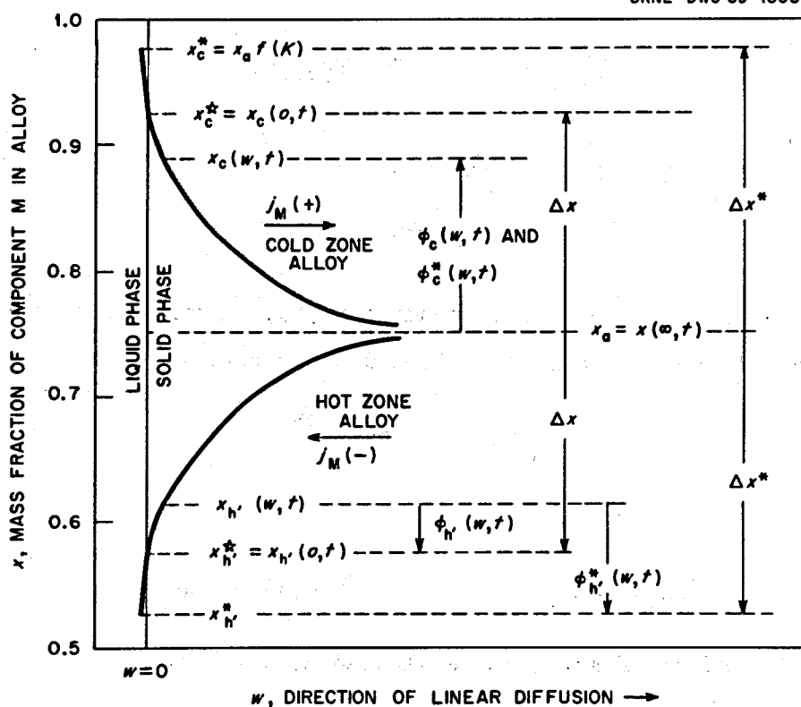
Fig. 1. The Relative Positions of Various Concentration Parameters and Variables. These quantities govern the concentration profiles in the tubing walls under transient, then steady-state conditions; they control concentration profiles and the migration rates in the alloy. An individual representation of reaction rate contributions is not shown; thus the difference, \Delta x^* - \Delta x , relates directly to h or \bar{h} .
