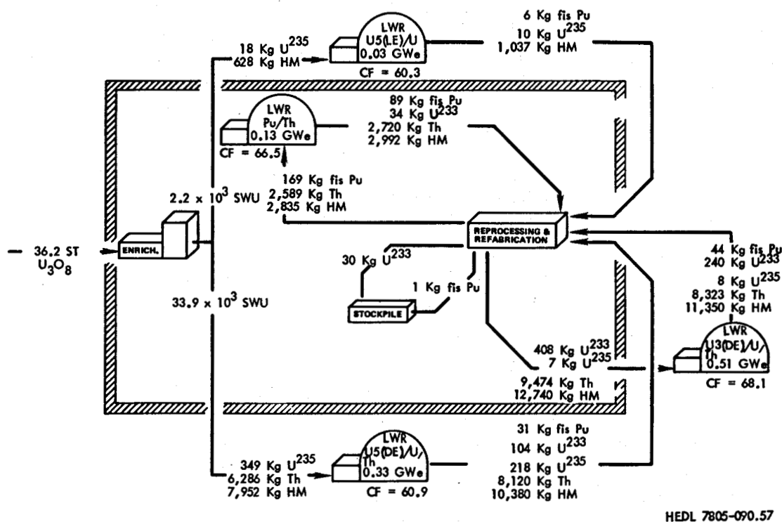
Fig. 6.2-24. Utilization and Movement of Fissile Material in an LWR Nuclear System Minimizing the Production and Use of Plutonium (Case 5UL, High-Cost U_3O_8 Supply) (Year 2035).
