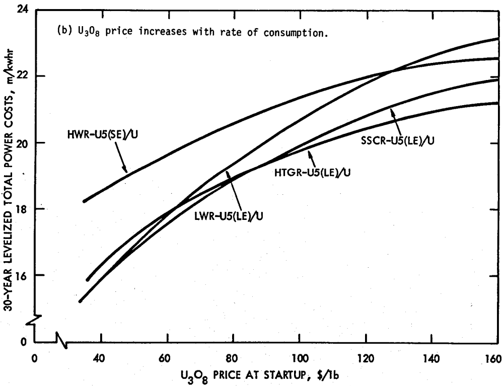
Fig. B-2. Effect of U_3O_8 Price on Total Power Cost for Reactors Operating on Throaway Cycle.
