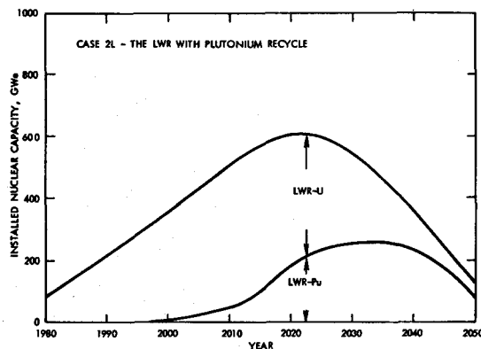
Fig. 6.2-14. Relative Nuclear Contributions of LWRs Located Inside (LWR-Pu) and Outside (LWR-U) Energy Centers (High-Cost U_3O_8 Supply).
