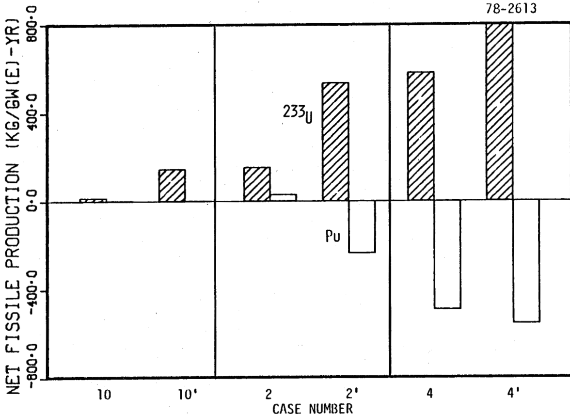
Fig. 4.6-2. Net Fissile Production Rates for LMFBRs. (Cases 10,10' for 233 U/Th core with no 238 U, Cases 2,2' for Pu/ 238 U core, and Cases 4,4' for Pu/Th core; see Tables 4.5-1 and 4.6-1.)
