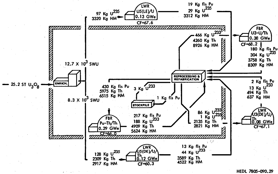
Fig. 6.2-35. Utilization and Movement of Fissile Material in an LWR-FBR Nuclear System with Heavy "Pu-to- ^{233}U ". Transmutation Rate (Case 8L, High-Cost U_3O_8 Supply) (Year 2035).
