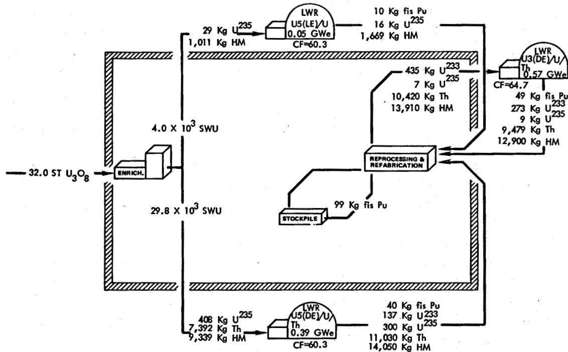
Fig. 6.2-19. Utilization and Movement of Fissile Material in a Nuclear System Consisting of LWRs Operating with Fissile Uranium Recycle and Plutonium Throwaway (Case 4L, High-Cost U_3O_8 Supply) (Year 2035).
