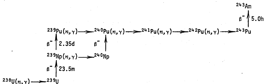
Fig. 4.0-2b. Nuclide Production Chain for ^{238}\text{U} .
