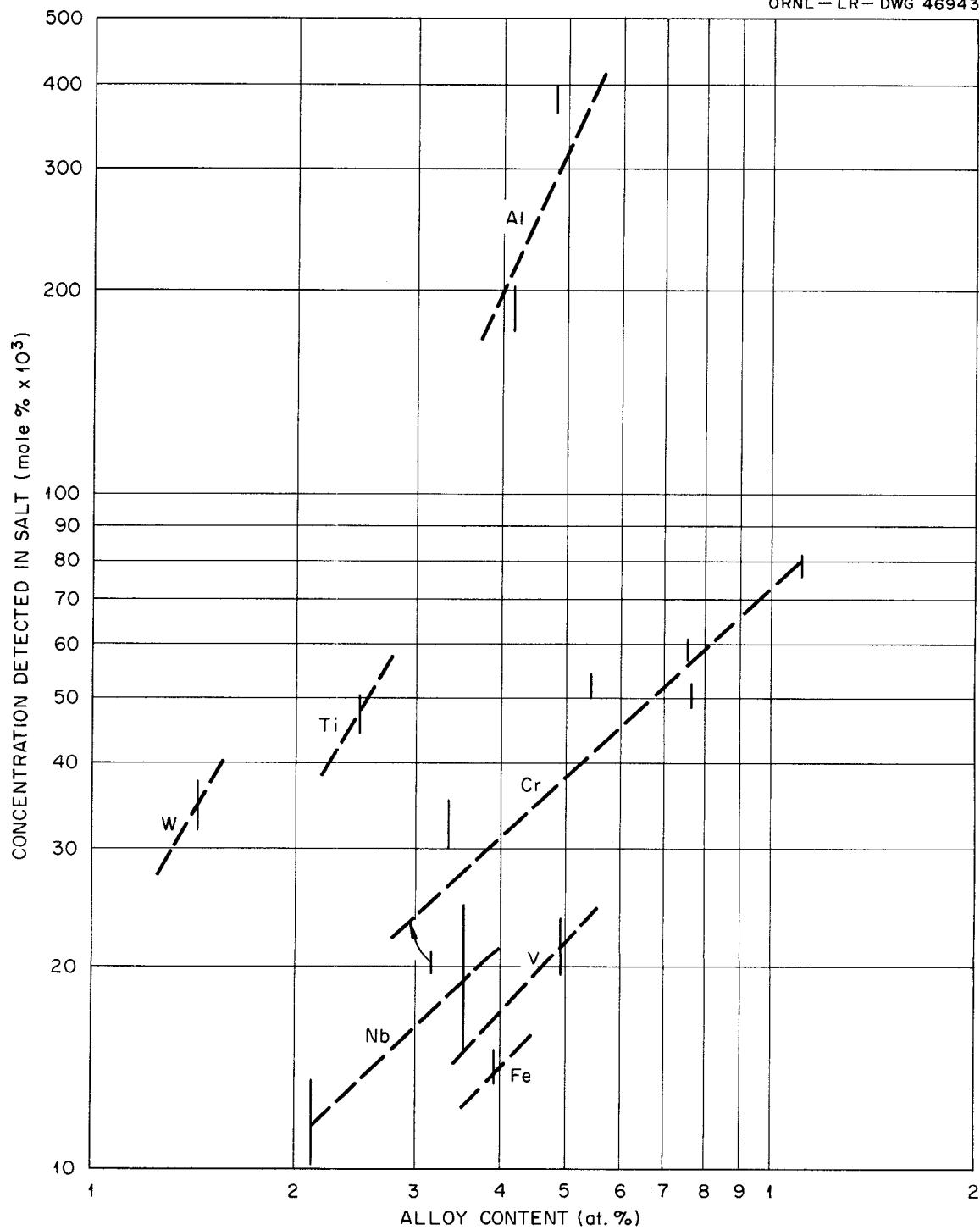
Fig. 13. Comparison of Corrosion-Product Concentrations Formed in Salt 107 by Various Alloying Additions as a Function of Alloy Content.
