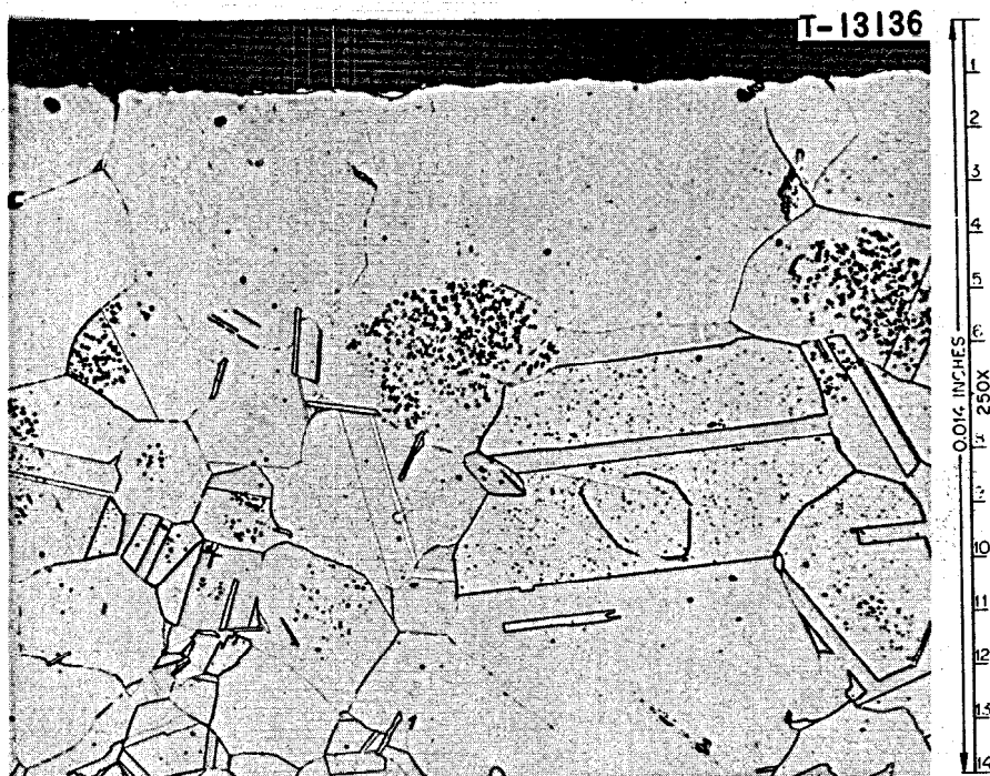
Fig. 11. Appearance of Voids in Nickel-Molybdenum Alloy Containing 3.62 at. % Nb after 1000-hr Exposure to Salt 107. Heat OR 30-21.
