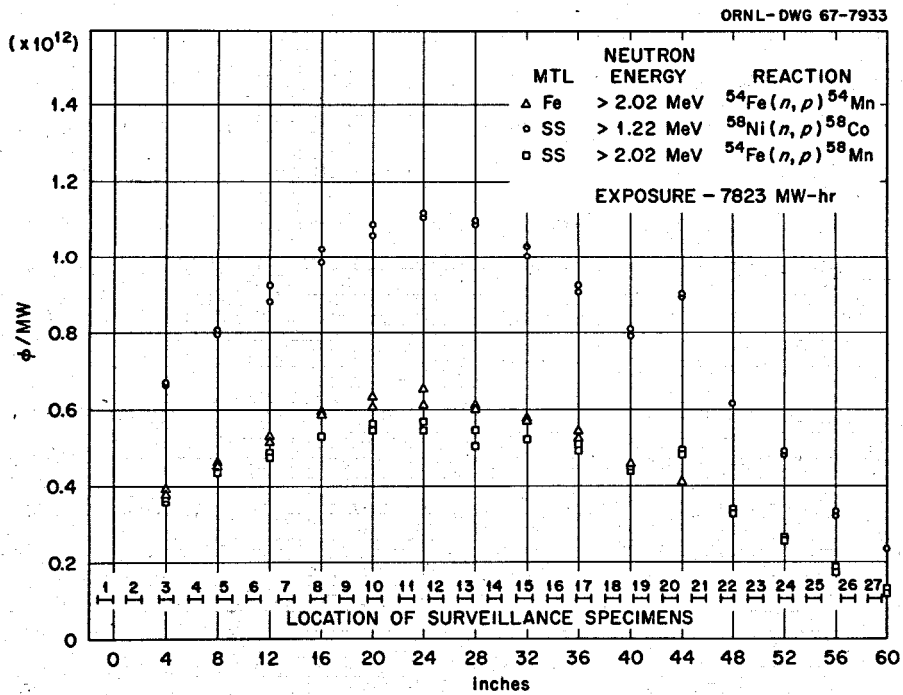
Fig. 3. Measurements of the Fast Flux for the MSRE Core Specimens - First Group.
