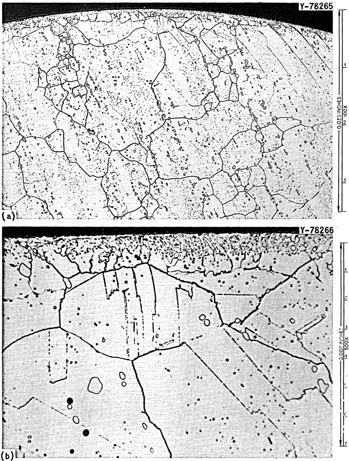
Fig. 32. Photomicrographs of the Cross Section of the Buttonhead of Specimen DC-25. (a) 100 x. (b) 500 x. Etchant: glyceria regia.
