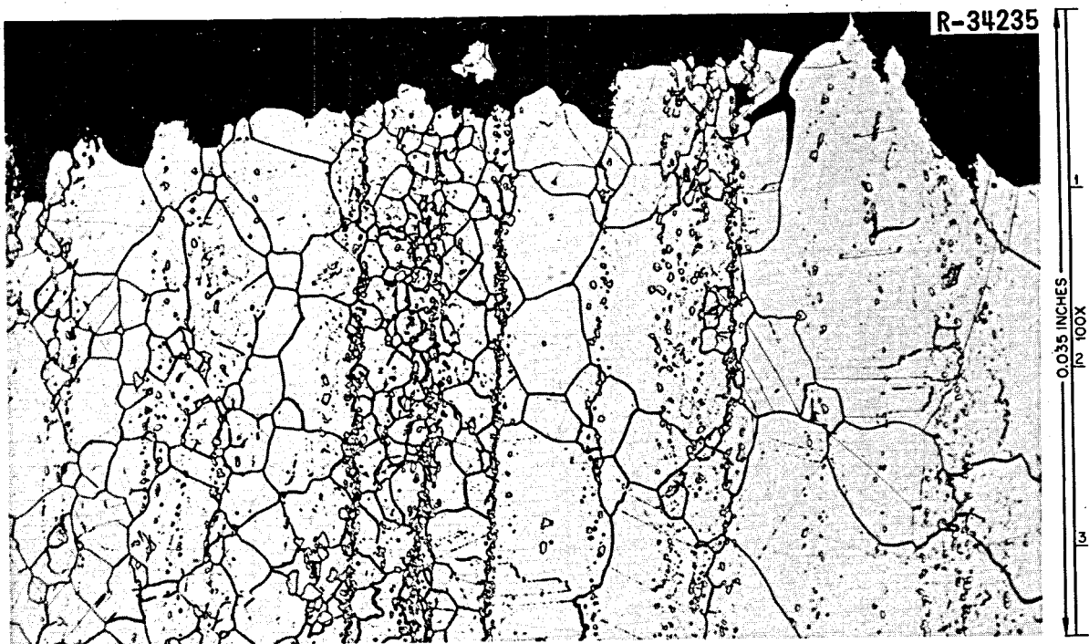
Fig. 27. Fracture of Surveillance Specimen E-14 from Heat 5081 Tested at 650^{\circ}\text{C} and at a Strain Rate of 0.002 \text{ min}^{-1} . Etchant: glyceria regia.
