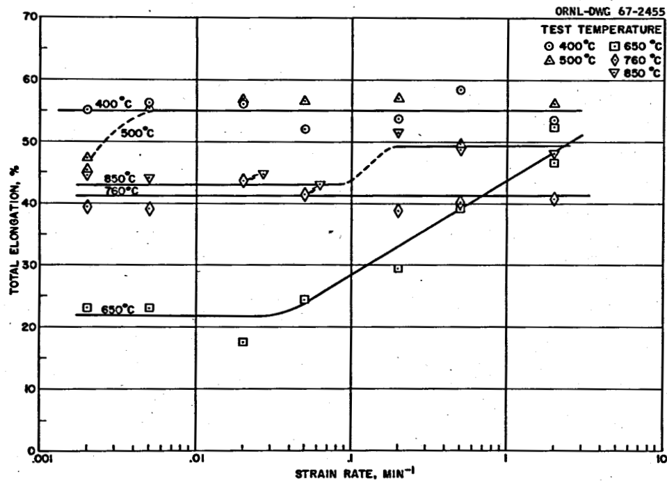
Fig. 5. Influence of Strain Rate on the Ductility of MSRE Surveillance Control Specimens, Heat 5081.
