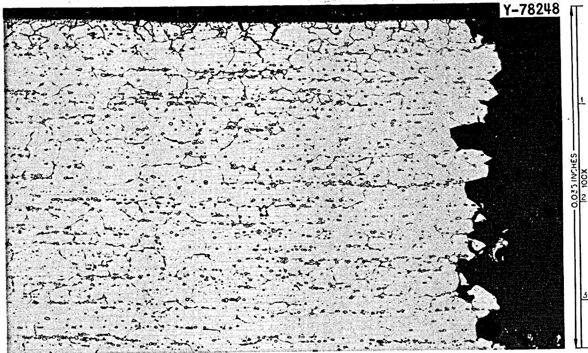
Fig. 26. Photomicrograph of the Fracture of Control Specimen AC-17 from Heat 5081 Tested at 650^{\circ}\text{C} and at a Strain Rate of 0.002 \text{ min}^{-1} . Etchant: glyceria regia.
