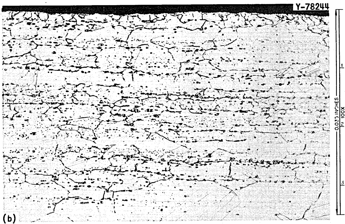
Fig. 24. Photomicrographs of Control Specimen AC-8 from Heat 5081 Tested at 25°C, and at a Strain Rate of 0.05 \text{ min}^{-1} . (a) Fracture. (b) Edge of specimen about 1/4 in. from fracture. Etchant: glyceria regia.
