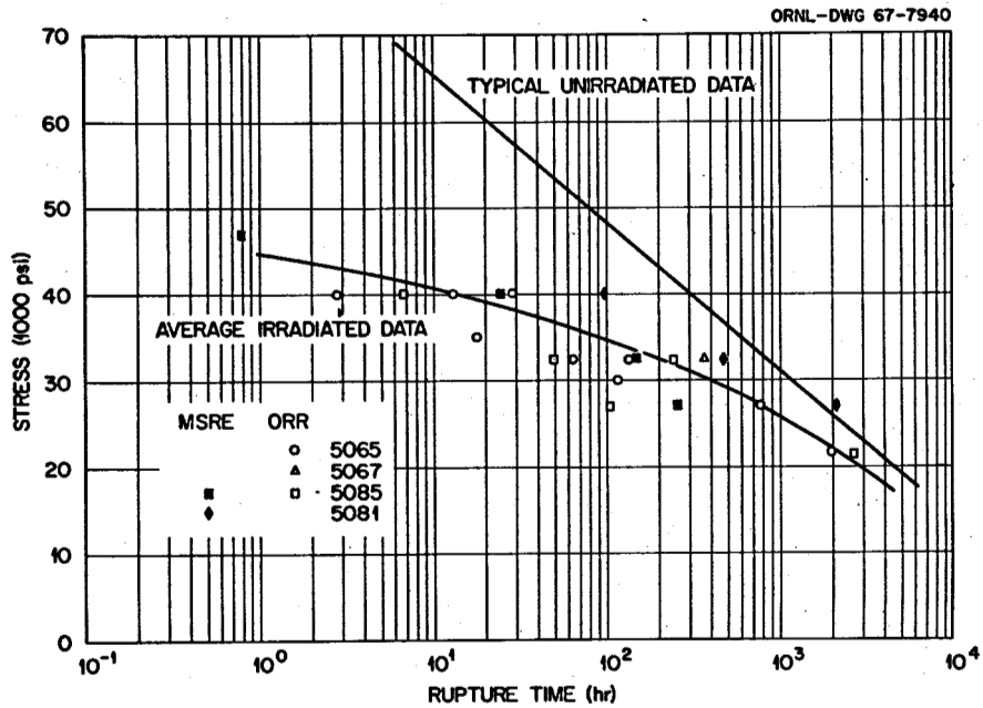
Fig. 22. Comparative Stress-Rupture Properties for Material Irradiated in the MSRE and the ORR at 650°C.
