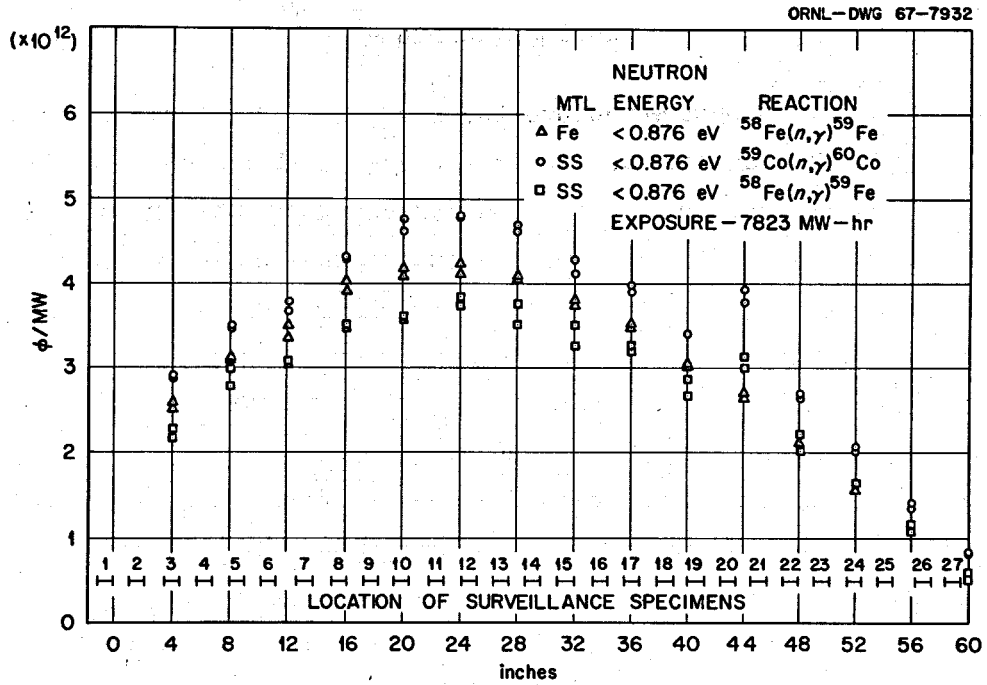
Fig. 2. Measurements of the Thermal Flux for the MSRE Core Specimens - First Group.
