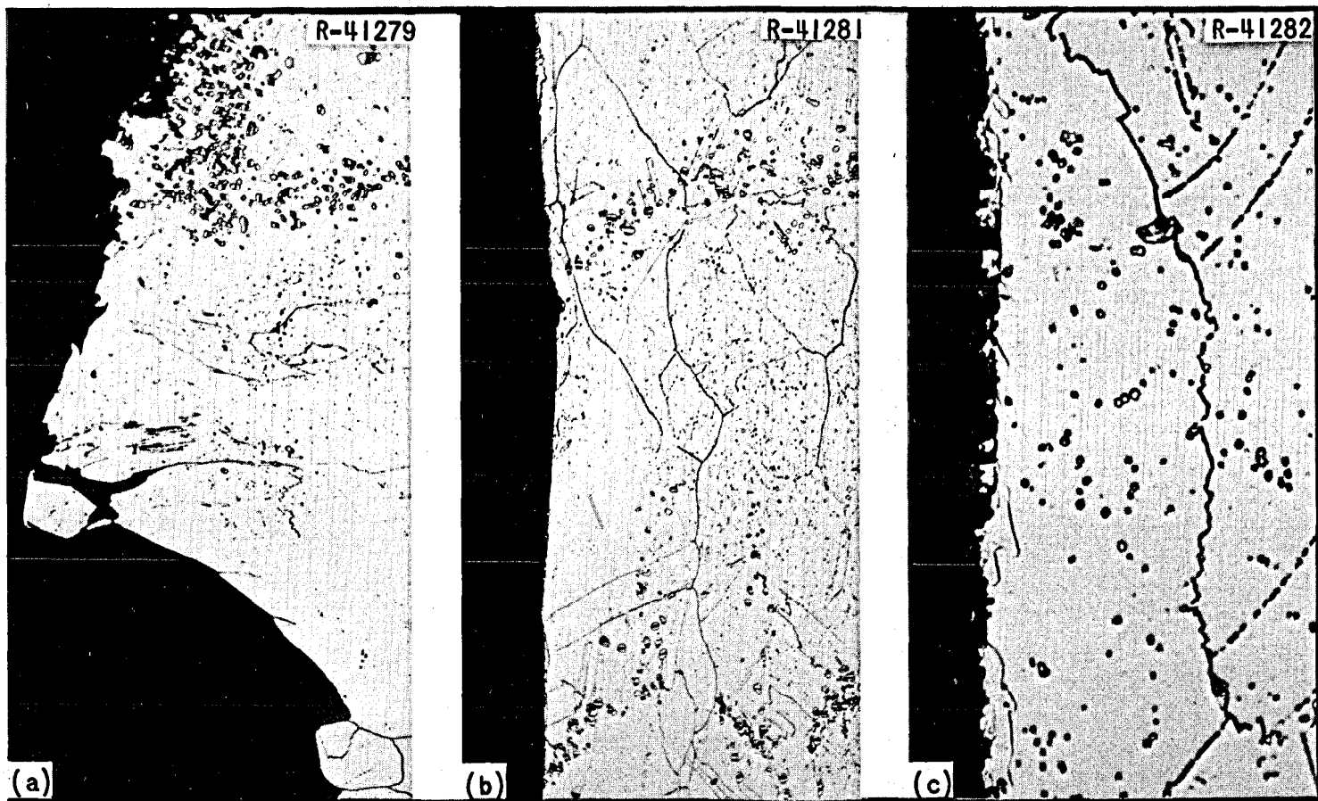
Fig. 28. Photomicrographs of a Hastelloy N Surveillance Sample (Heat 5065) Tested at 25°C at a Strain Rate of 0.05 min -1 . Exposed outside the core for 11,000 hr at 650°C to a thermal fluence of 1.3 \times 10^{19} neutrons/cm 2 . Etchant: Aqua regia. (a) Fracture - note the mixed transgranular and intergranular fracture. 100X. (b) Edge of sample about 1/2 in. from fracture. Note the fractured precipitates. 100X. (c) Edge of sample showing shallow surface oxidation and extensive precipitation. 500X.
