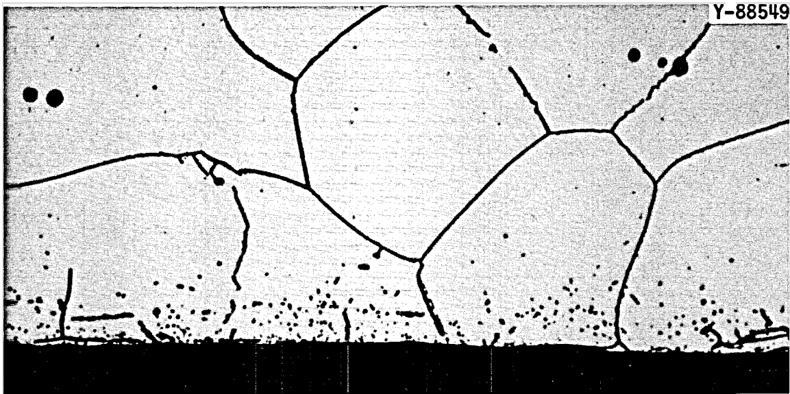
Fig. 9. Photomicrograph of the Material Used to Make the Surveillance Basket after a 1-hr Anneal at 1177°C and Aging for 1000 hr at 650°C. 750 \times . Etchant: Glyceria regia.
