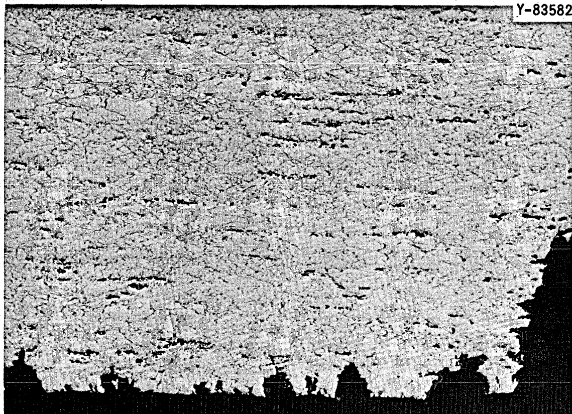
Fig. 37. Photomicrograph Showing a Portion of the Fracture of a Zirconium-Modified Hastelloy N Sample (Heat 21554) Tested at 650°C at a Strain Rate of 0.002 min -1 . Exposed to static fluoride salt for 5500 hr at 650°C before testing. 100X. Etchant: Glyceria regia.
