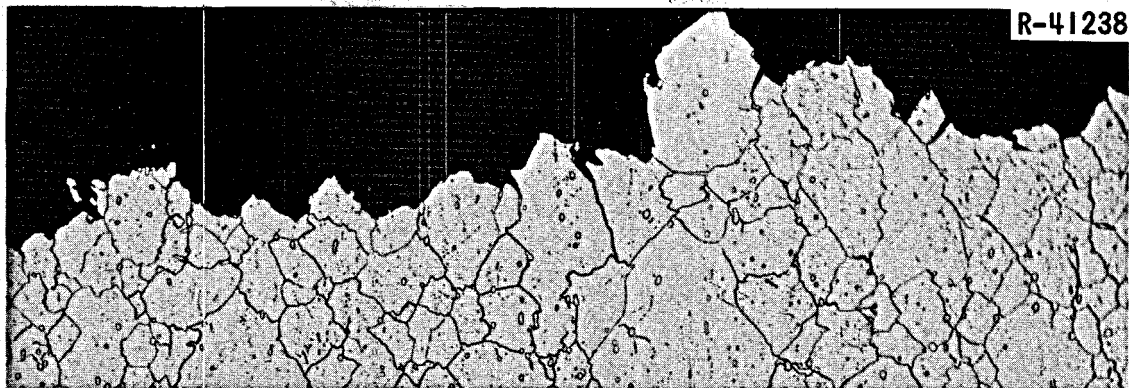
Fig. 29. Photomicrograph of the Fracture of a Standard Hastelloy N Surveillance Sample (Heat 5065) Tested at 650°C at a Strain Rate of 0.002 min -1 . Exposed outside the core for 11,000 hr at 650°C to a thermal fluence of 1.3 \times 10^{19} neutrons/cm 2 . 100X. Etchant: Aqua regia.
