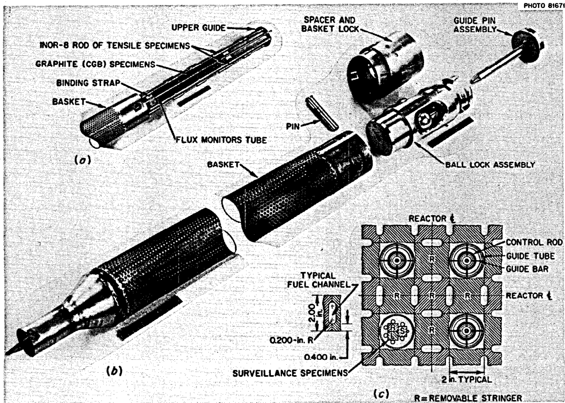
Fig. 1. Molten-Salt Reactor Experiment Core Surveillance Fixture.
