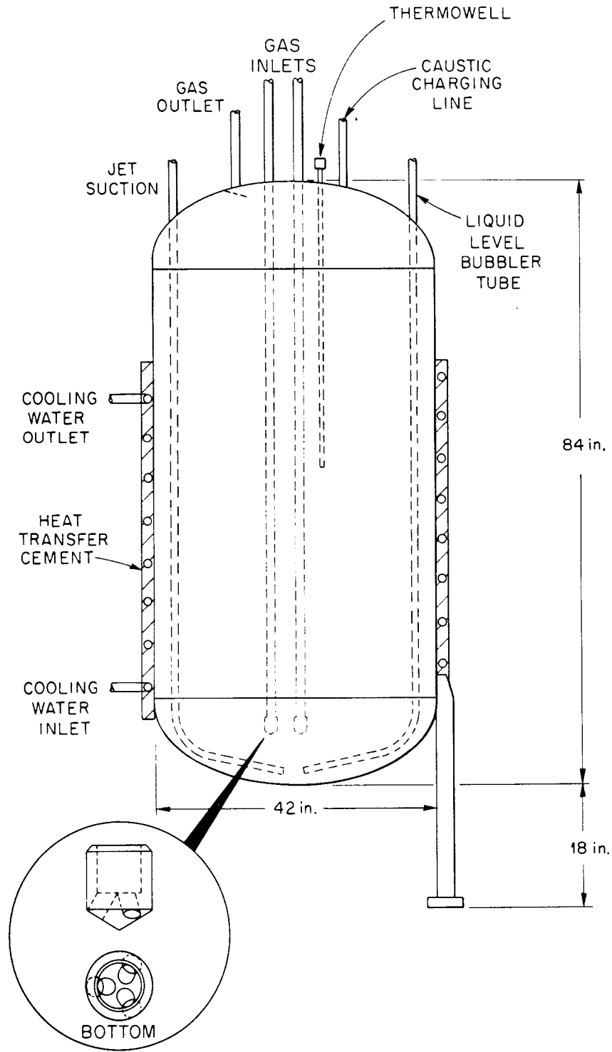
Fig. 7. Caustic Scrubber.
