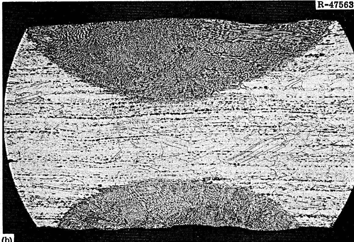
Fig. 2. Photomicrographs of Sample 10,082. Heat 5085, Unirradiated, welded in the hot cell and tested at 25°C. Fracture occurred in the base metal. (a) As polished. (b) Etchant: glyceria regia. 35X.
