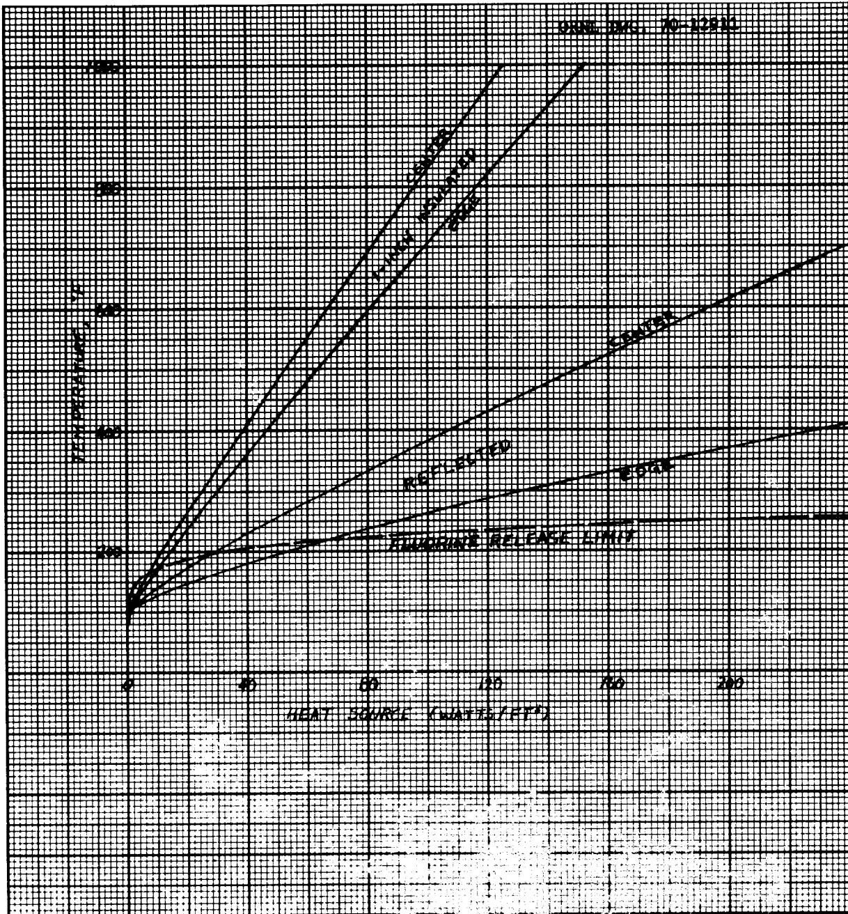
Fig. 9. Temperatures in Insulated 2-ft Diameter Cans of Salt in 100°F Air and the Temperature Required to Prevent Fluorine Release
