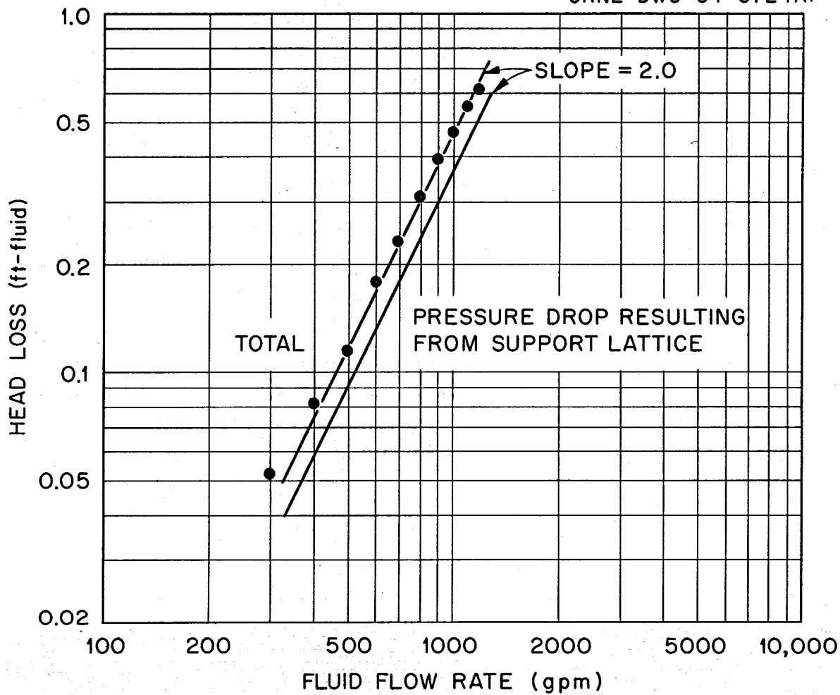
FIGURE 12. FUEL SALT PRESSURE DROP ACROSS MODERATOR ASSEMBLY
