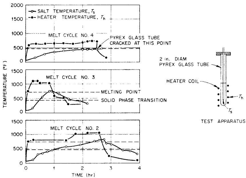
Fig. E.1. Data from fluoroborate freeze-thaw stress test.
