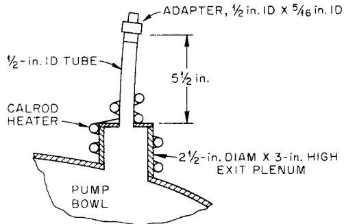
DETAIL OF PUMP BOWL OFF-GAS NOZZLE-TESTS Ia TO Ic
