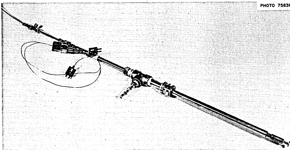
Fig. 17. Cold-finger assembly.
