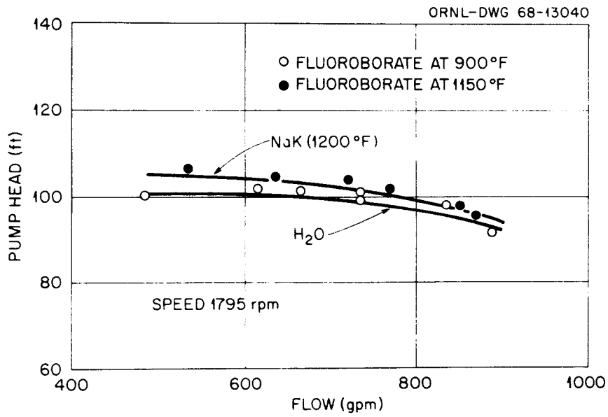
Fig. 11. Comparison of PKP pump characteristics with sodium fluoroborate, NaK, and water.
