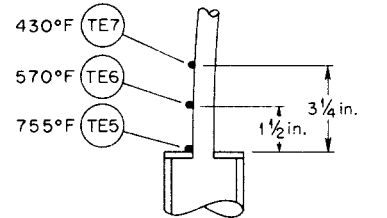
TYPICAL TEMPERATURE PROFILE WITH CALROD HEATER TURNED OFF
