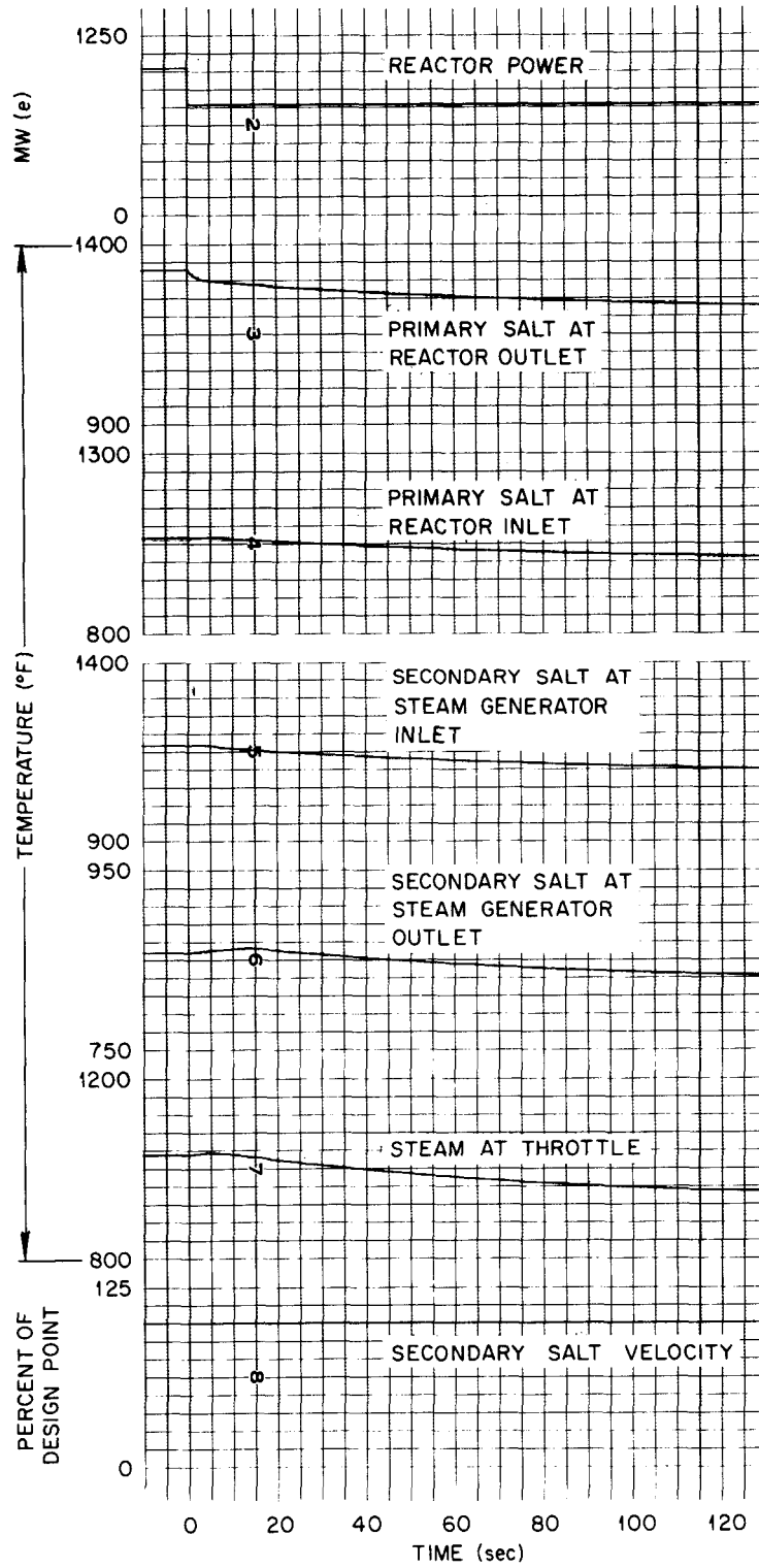
Fig. 9. System Response to a Step Change in Nuclear Fission Power from 100 to 75%.
