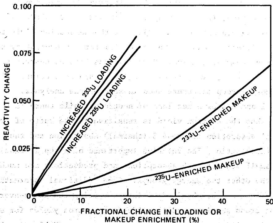
Fig. 6. Effect of initial loading and enriched makeup on equilibrium reactivity.
